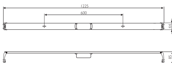
Technical Drawing
