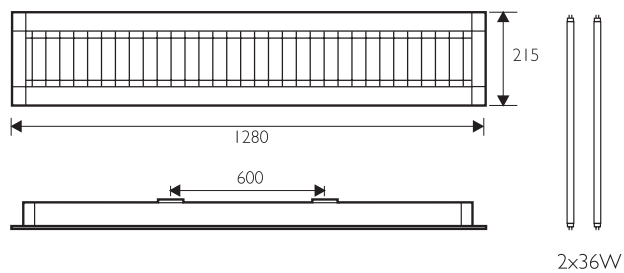
Technical Drawing
