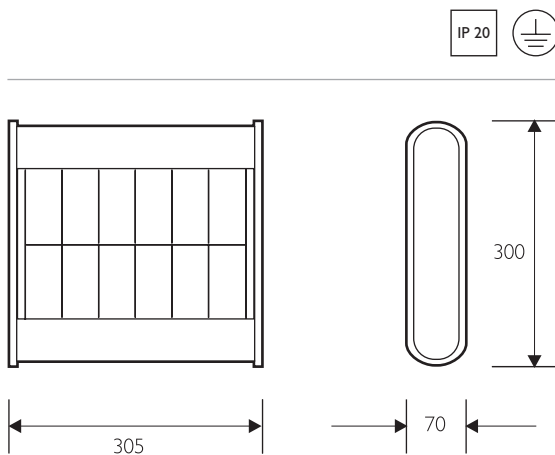
Technical Drawing
