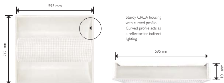
Dimensional details
