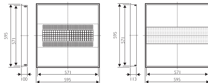
Technical Drawing
