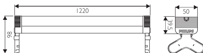
Technical Drawing
