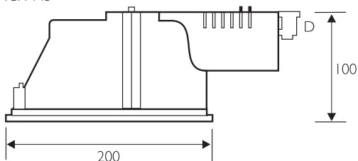
Technical Drawing
