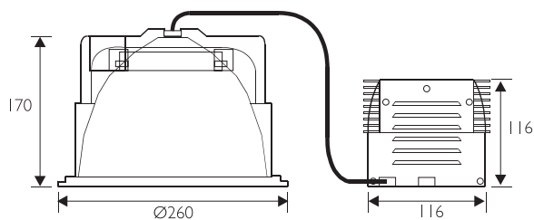
Technical Drawing
