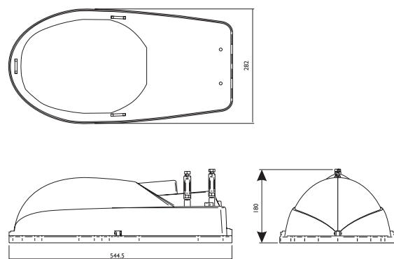
Technical Drawing
