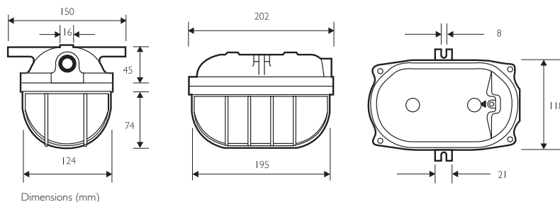
Technical Drawing
